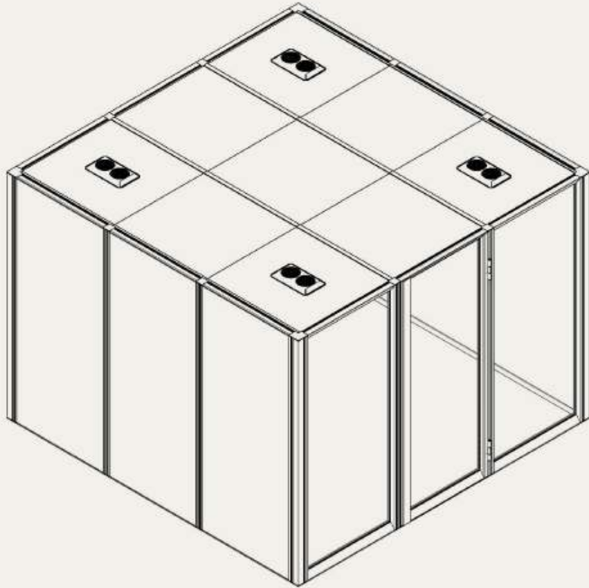
Solid ceiling modules with ventilation system
