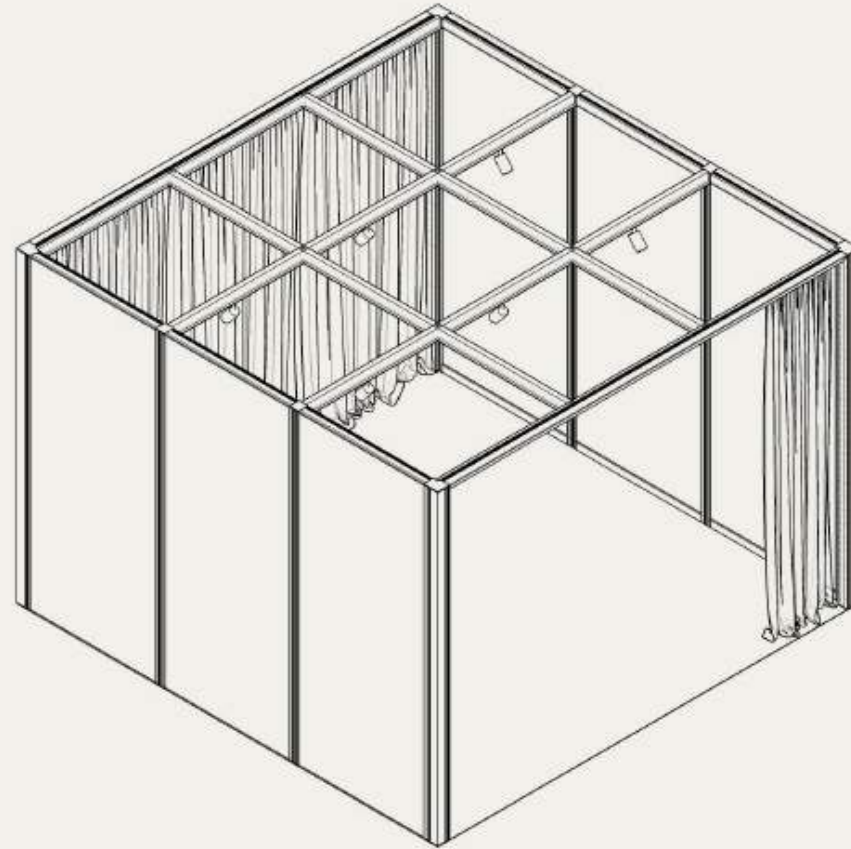
Openwork ceiling with front overhanging beam
